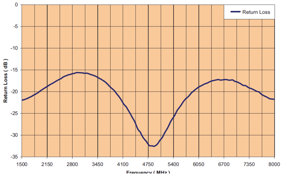
RFLM-202802LC-299 Return Loss vs Frequency
