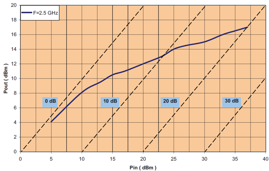
RFLM-202802LC-299 P_{out} vs P_{in} Function CW
