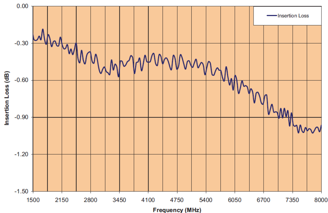
RFLM-202802LC-299 Insertion Loss vs Frequency
